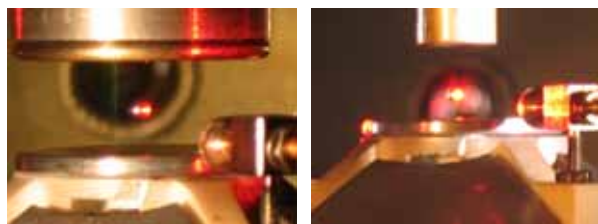
Fig.2 Actual electrodes arrangement in the JAXA electrostatic levitator; past(left) and present (right).
